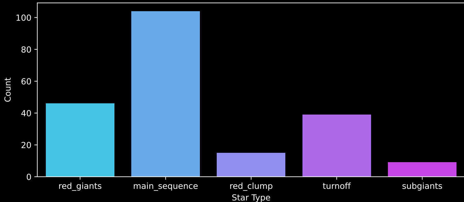
APOGEE DR17 Field: [268-39-O_TESS] Count plot of Star Type
